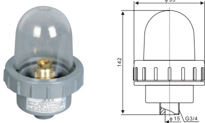
CXH5-2A 桅顶灯 Head light
