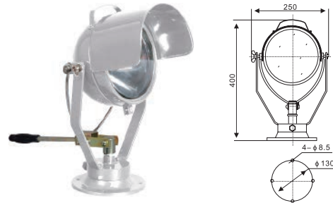
搜索灯 TG16B Search light
