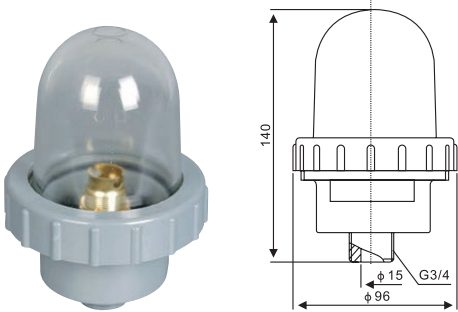
CXH5-2 桅顶灯 Head light
