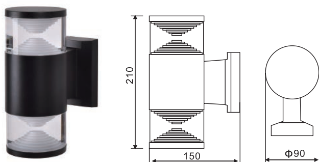
CBD2 壁灯 Wall light
