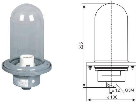
CXH5-1 桅顶灯 Head light
